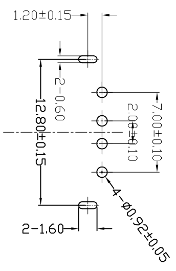
FRONT EDGE OF CONNECTOR PCB LAYOUT (T=1.60mm)
